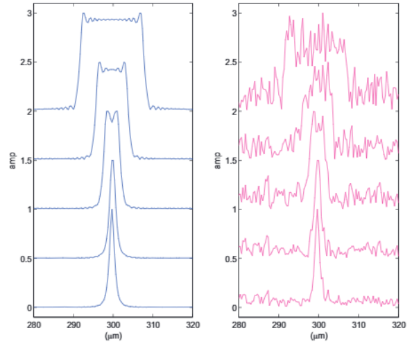
Fig. 5. (a) Implementation of a CW light source of various widths ( w ) in vacuum. (b) Implementation of a CW light source of various widths ( w ) embedded in a scattering medium (from bottom to top) w = 1, 2, 4, 8 , and 16 \mu\text{m} , respectively. The scattering medium consists of 800 6- \mu\text{m} -diameter, dielectric ( n = 1.2 ) cylinders clustered in a region of 180- \mu\text{m} -radius. The amplitude profile (measured along the white dashed line of Fig. 1) is more complex due to interference of light reflected and refracted from the scattering medium.
