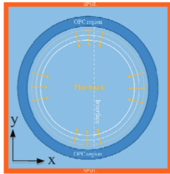
Fig. 6. CW light recorded in the forward propagation is phase-conjugated and added into the OPC region (the blue shaded region) as a soft source.
